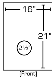
Counter-Top Drain Hole Location
